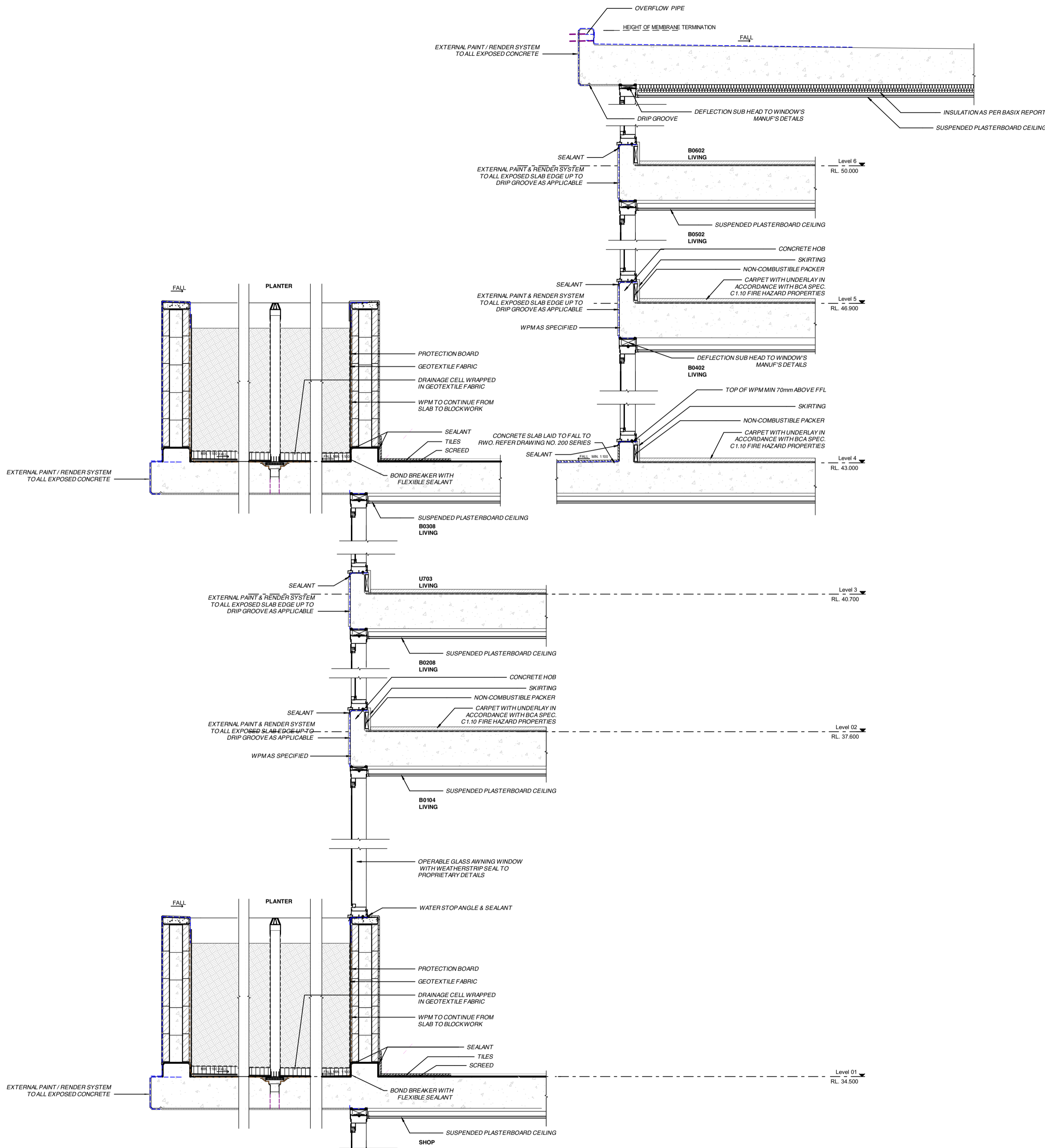
1 Building B Section Through Shop & Units 1:20
